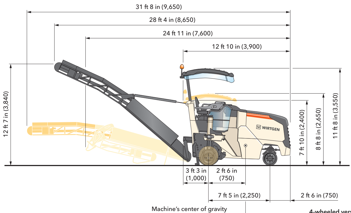
4-wheeled version
