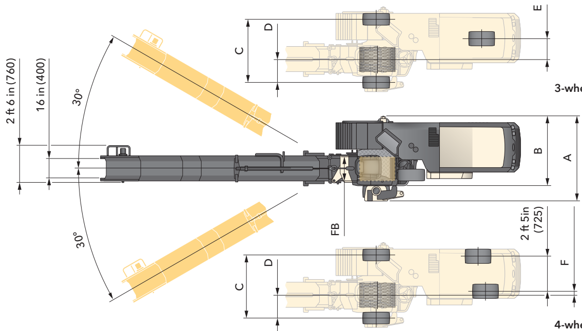
4-wheeled version
